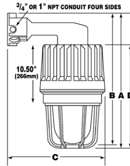
Wall Bracket
