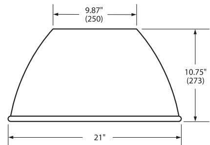
Deep Dome
