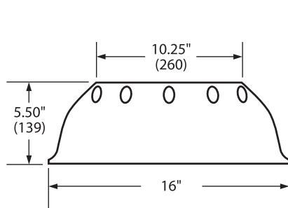
Standard Dome
