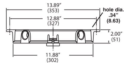
Ceiling Mount
