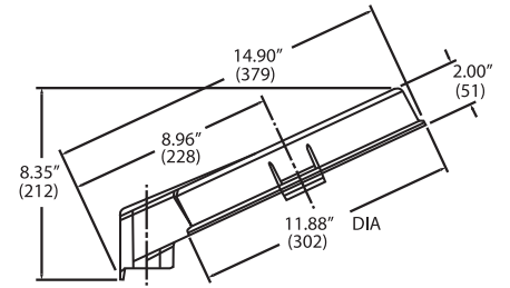
Stanchion(25°) Mount
